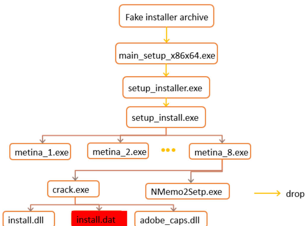
Execution flow, variant 2
