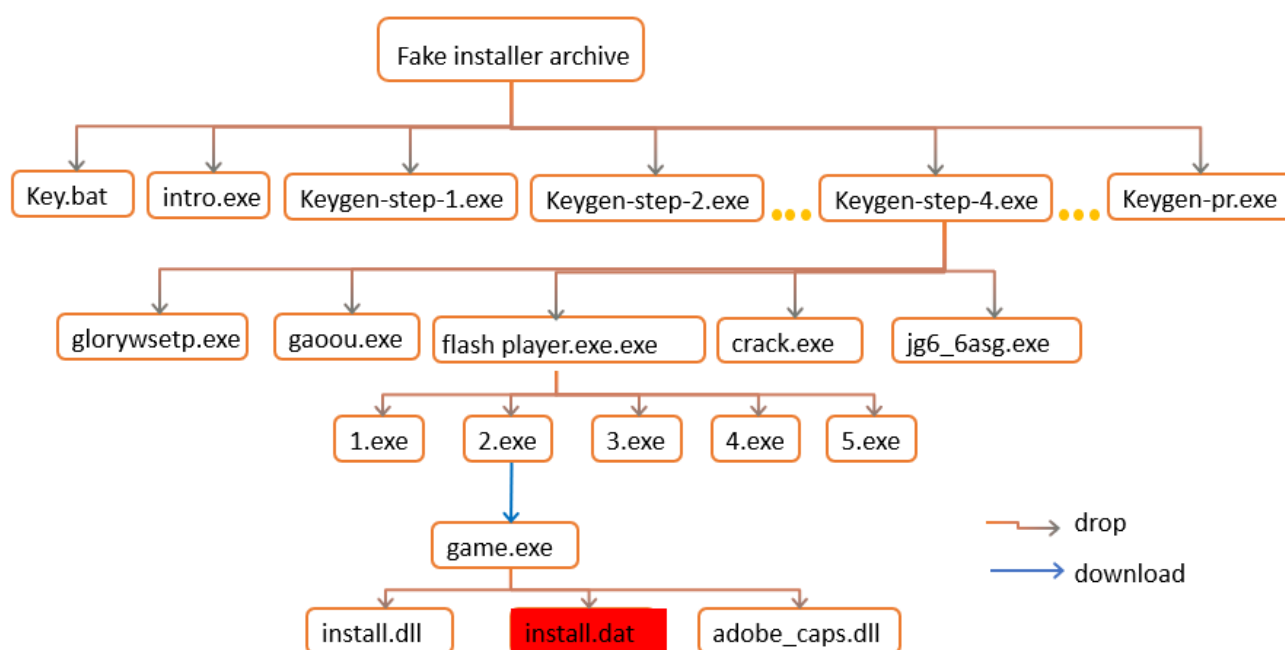
Execution flow, variant 1
